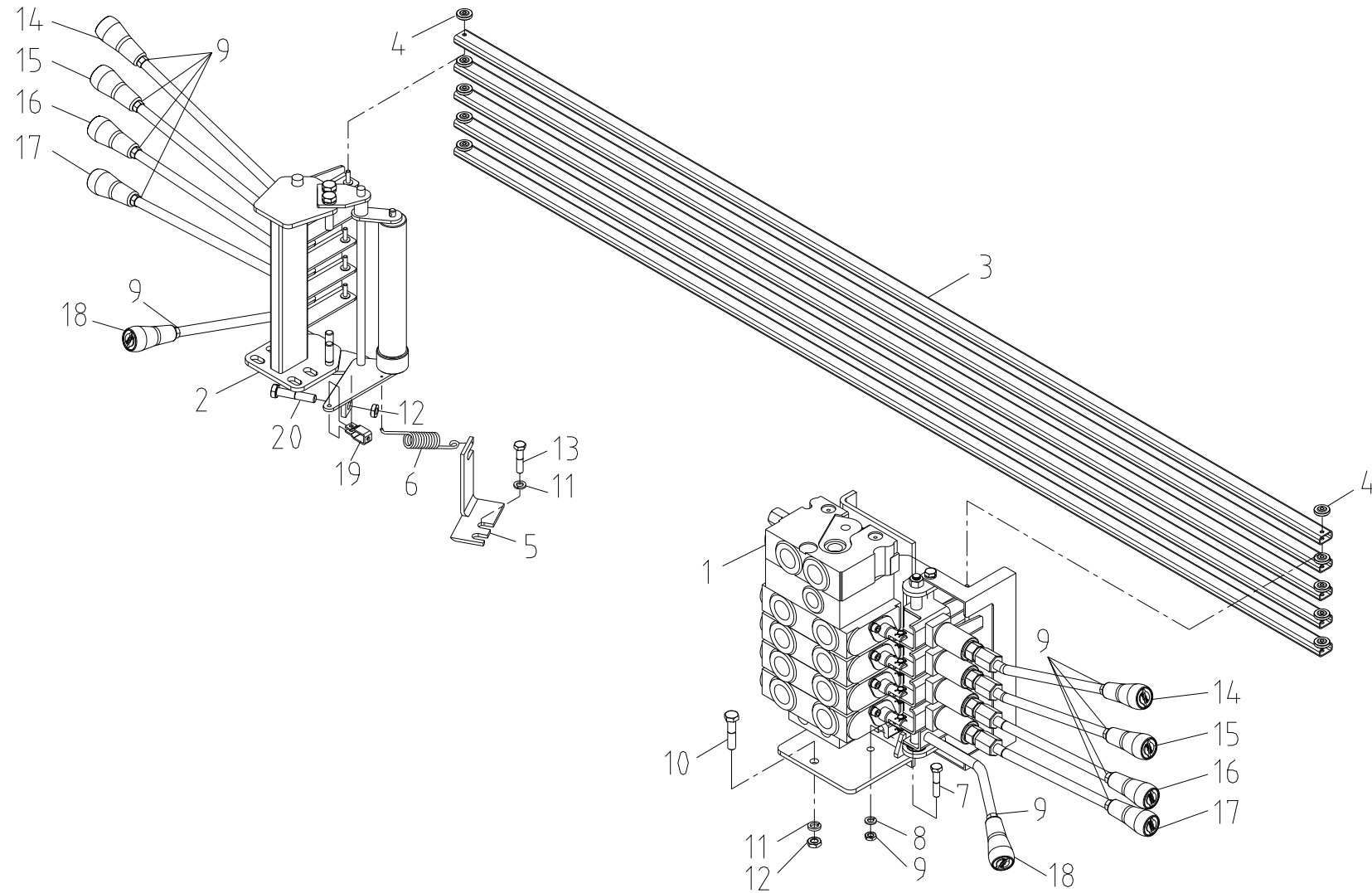
Fig. 3-5 SCS323 OPERATION MAIN ASS'Y(II)
